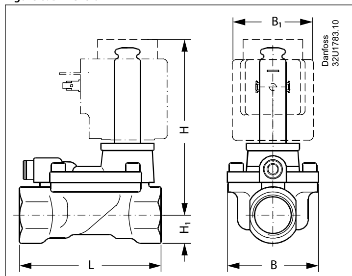
Figure 6: Dimension
