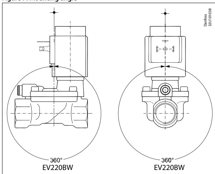
Figure 7: Mounting angle
