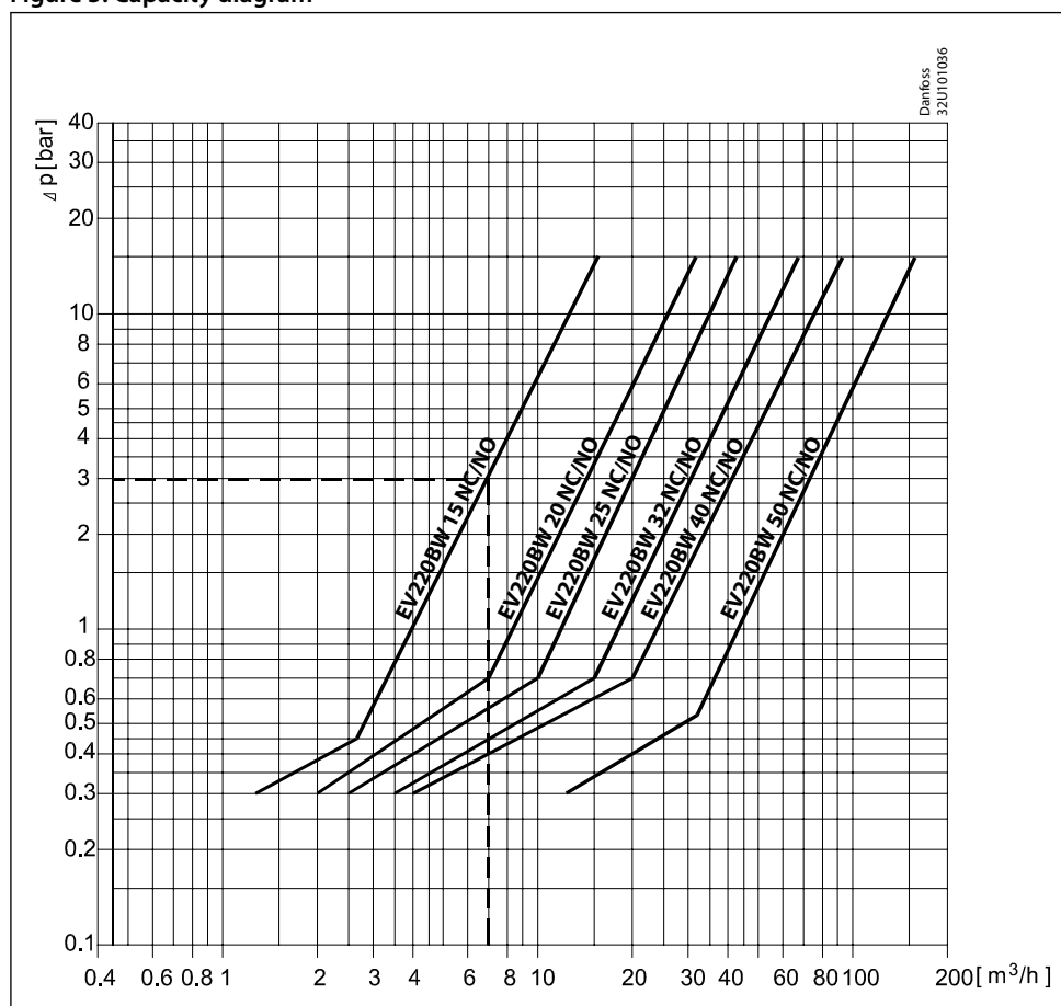
Figure 5: Capacity diagram
